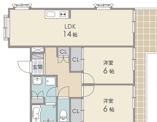
A type 2LDK 65.29 m 2 (19.75 坪)
